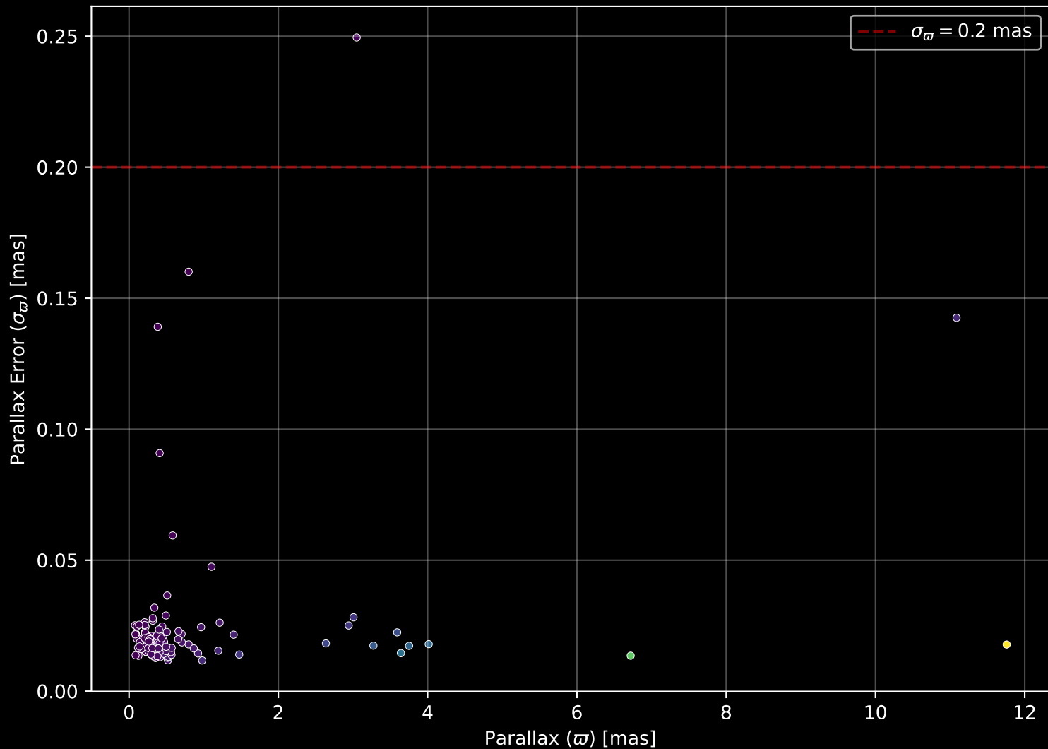
APOGEE DR17 Field: [135-06] Parallax Quality (n= 156)
