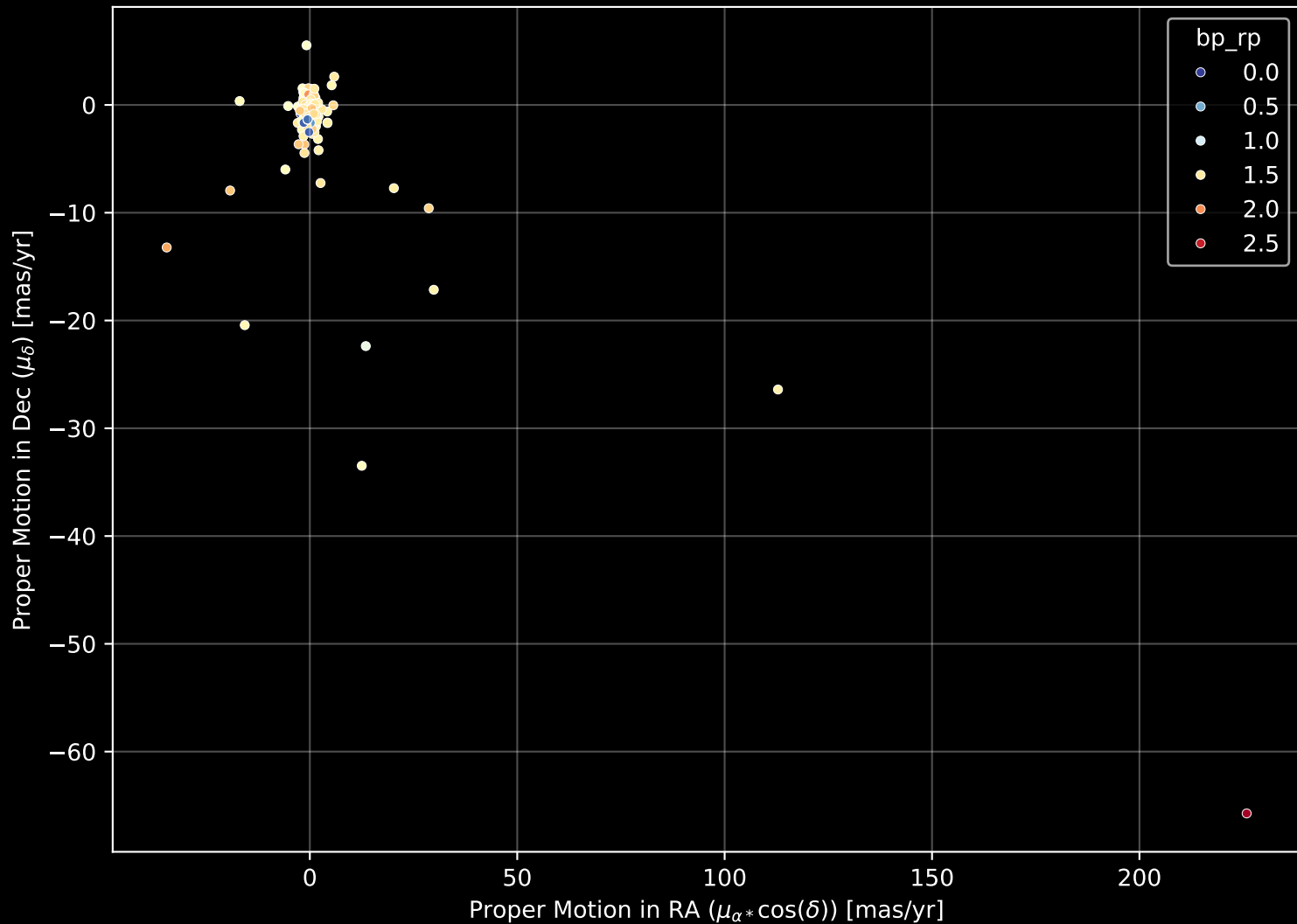
APOGEE DR17 Field: [135-06] Proper Motion Diagram (n= 156)
