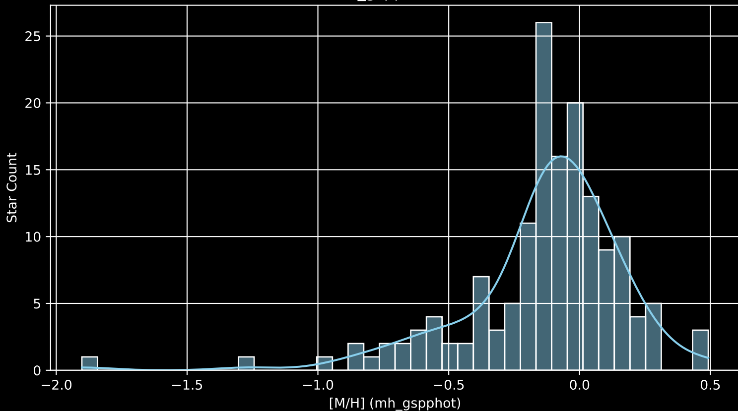
APOGEE DR17 Field: [135-06 [M/H] (mh_gspphot) (n= 153)
