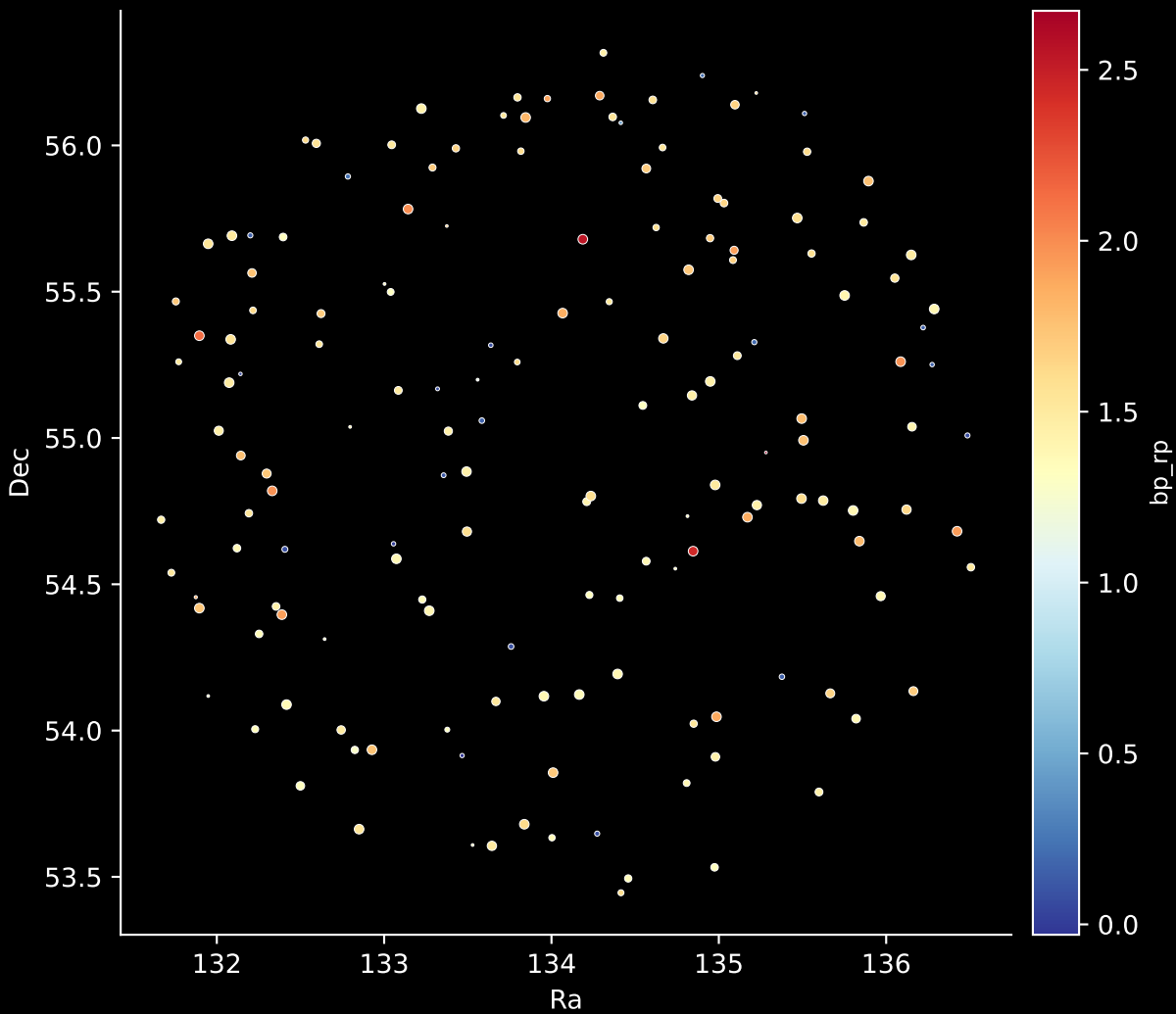
APOGEE DR17 Field: [135-06] Stars: 156
