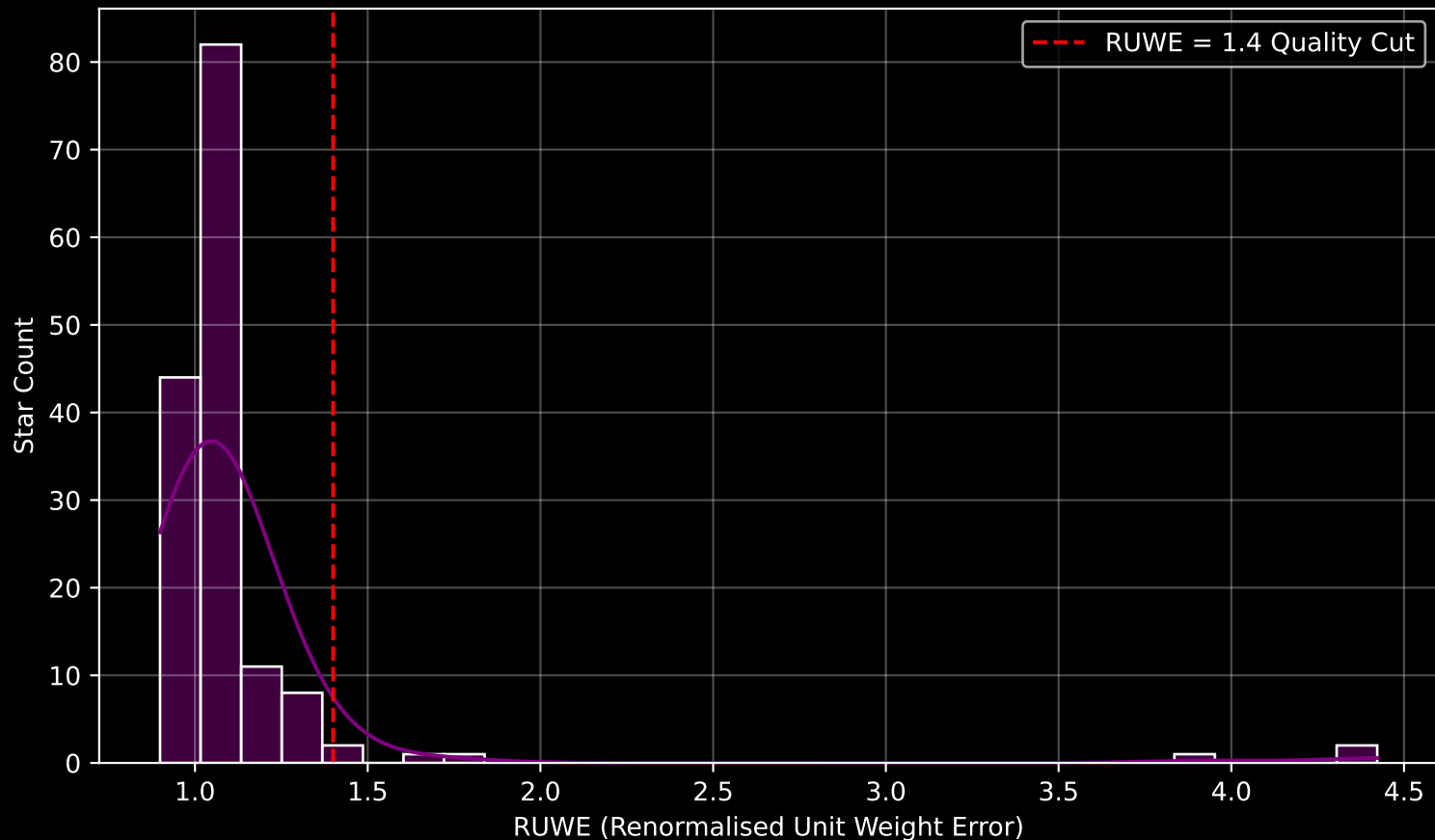
GAPOGEE DR17 Field [135-06] RUWE Distribution (n= 152)
