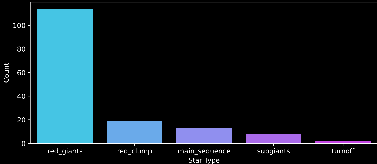
APOGEE DR17 Field: [135-06] Count plot of Star Type
